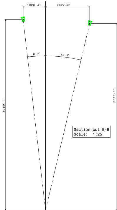
EQUATORIAL ELM COIL
