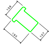
Detail S Scale: 1:5 ELM COIL SECTION
