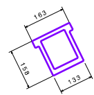
Detail R Scale: 1:5 VS COIL SECTION
