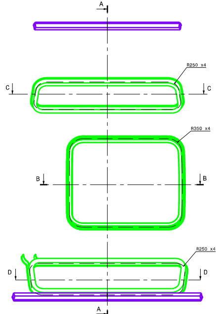
Front view Scale: 1:25
